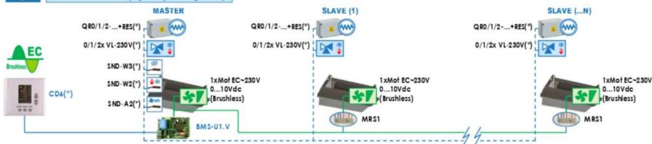
Fig.5 MASTER-SLAVE (Open-space System)
