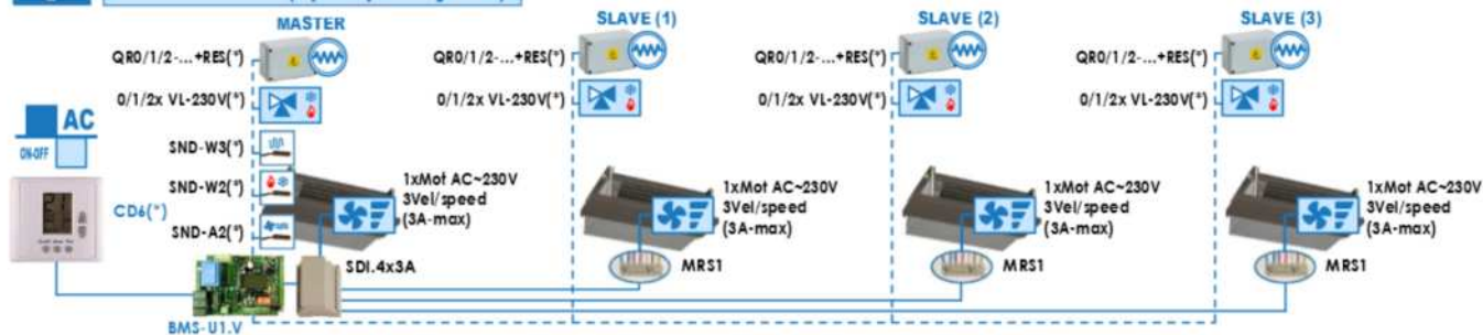
Fig.4 MASTER-SLAVE (Open-space System)
